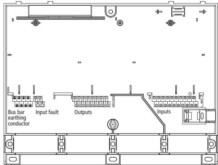
Inputs and outputs of the OT Box RAMSES top2 OT
